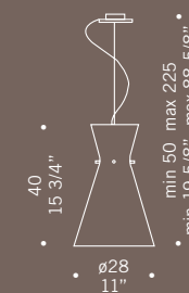
MEMORY SL 1x70W E27 alogena chiara clear halogen 1x150W E27 alogena chiara clear halogen 1x75W E27-PAR 30 1x30W E27 fluorescente fluorescent
