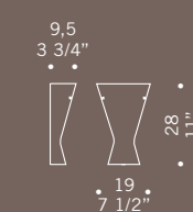
MEMORY A1 1x120W R7s alogena lineare 75 mm halogen linear 75 mm
